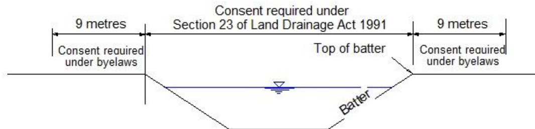
Open Watercourse without Embankments
