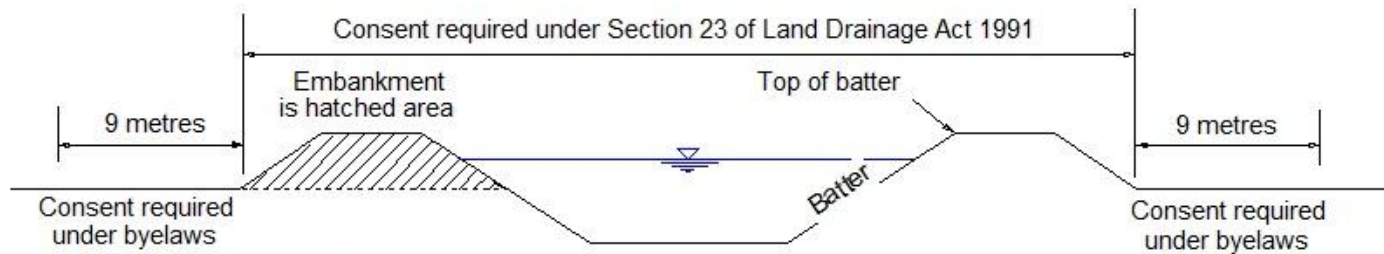
Open Watercourse with Embankments
